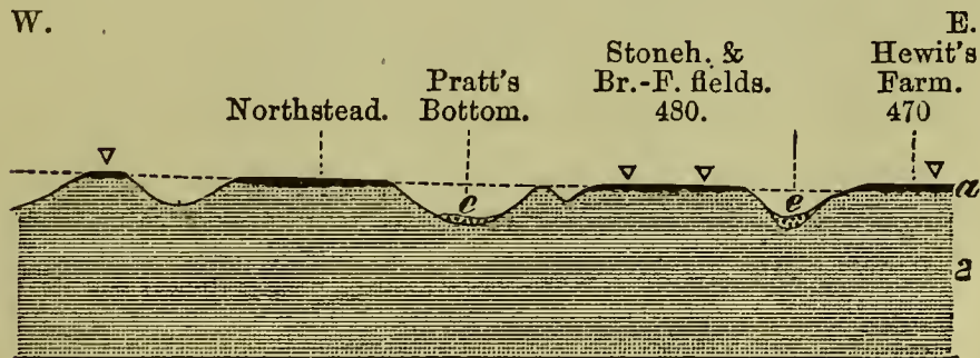
Fig. 3.—Transverse section (1) across the promontories.
